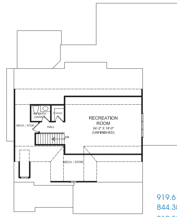
THIRD FLOOR
